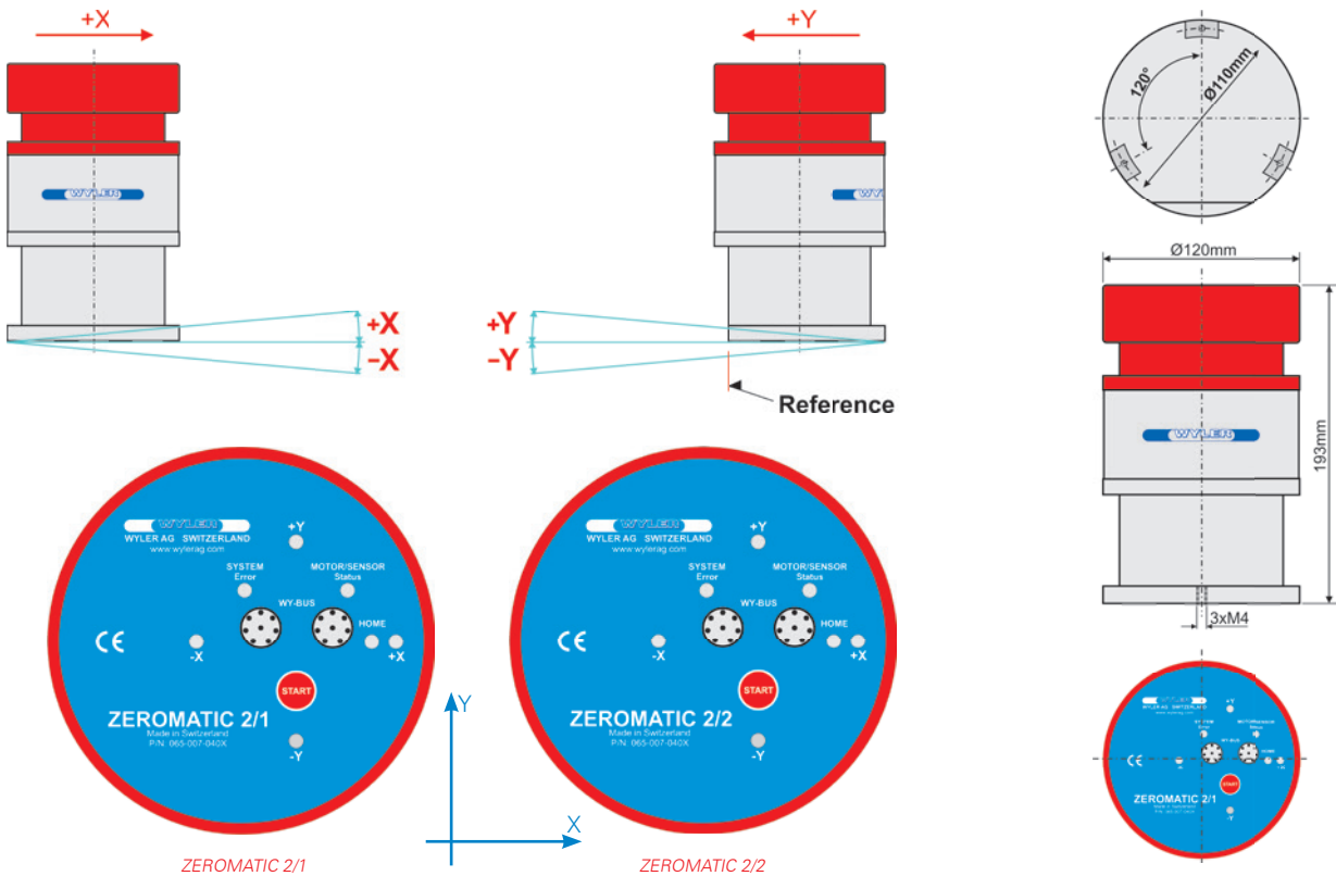
Outer dimensions of the ZEROMATIC sensor 2/1 and 2/2
