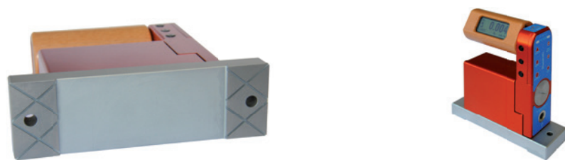
Base Type 122 Steel, hardened, contact surfaces flat, precision lapped, with dust grooves, remaining surfaces nickel-plated
